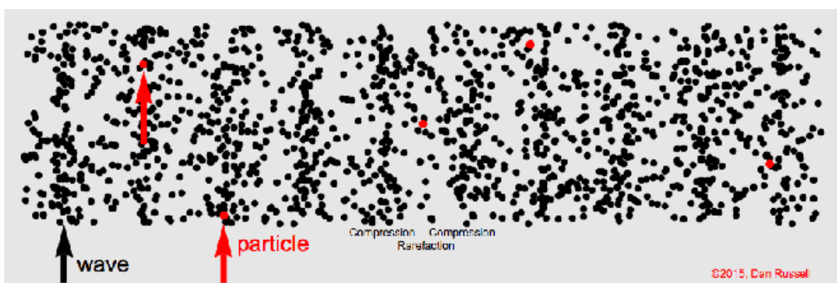
Wave and particle duality and illustration.
